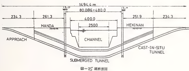
Fig. 2S Longitudinal Section of Tunnel
